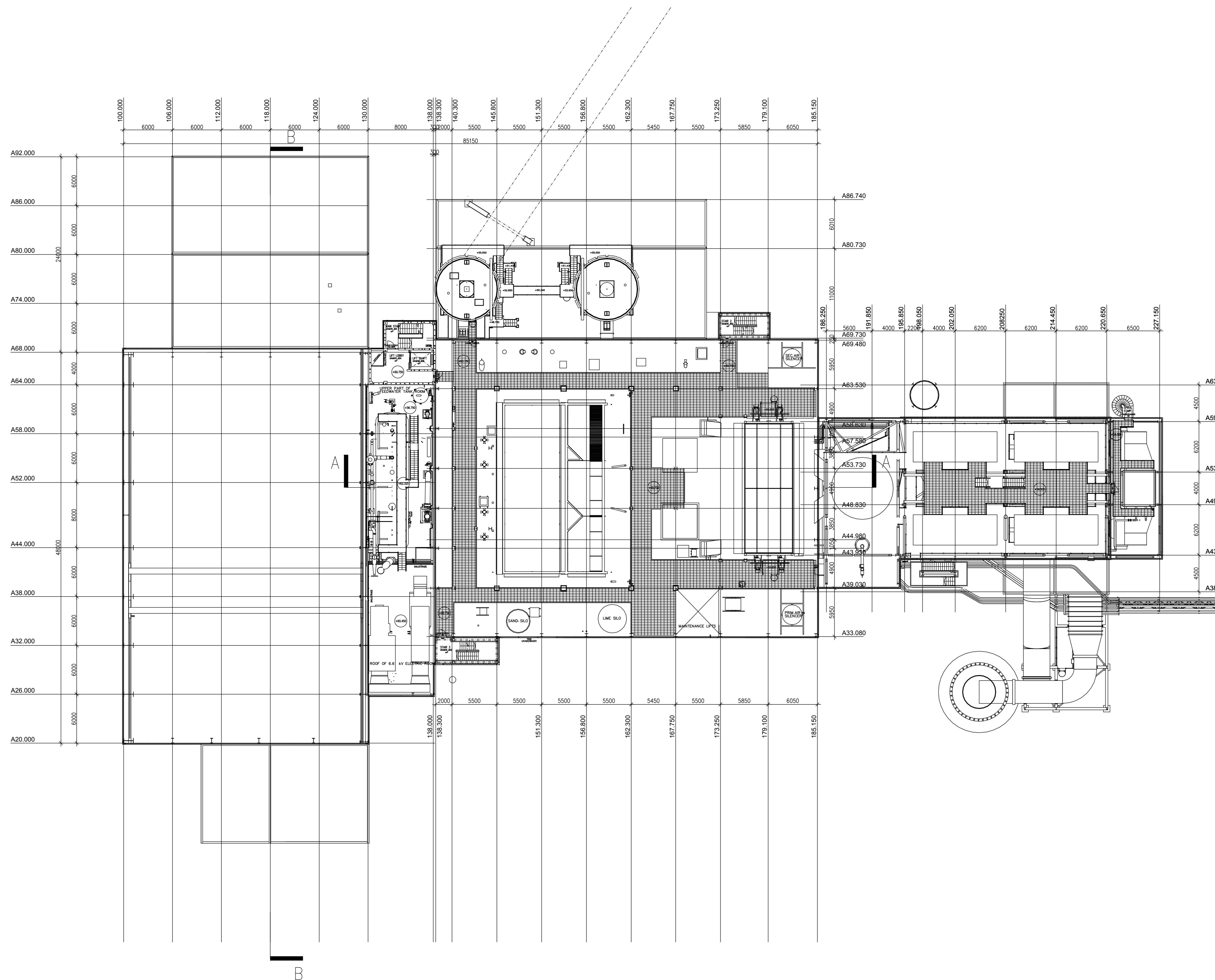
PLAN @ LEVEL +60.750m
